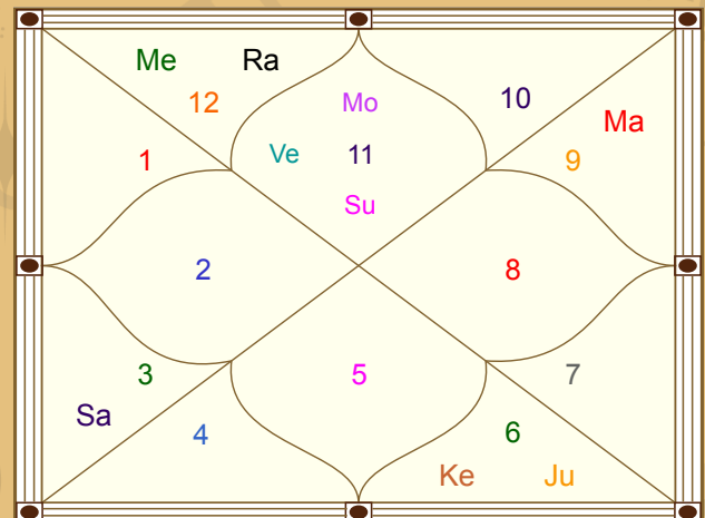
Sun Chart
