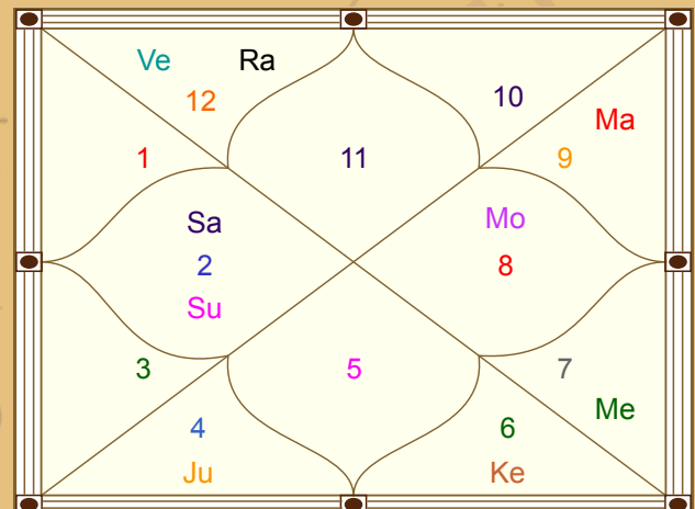
Navamsa Chart
